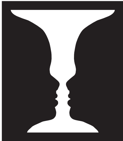
Rubin's Vase
