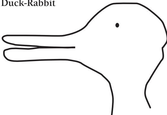
Jastrow's Duck-Rabbit
