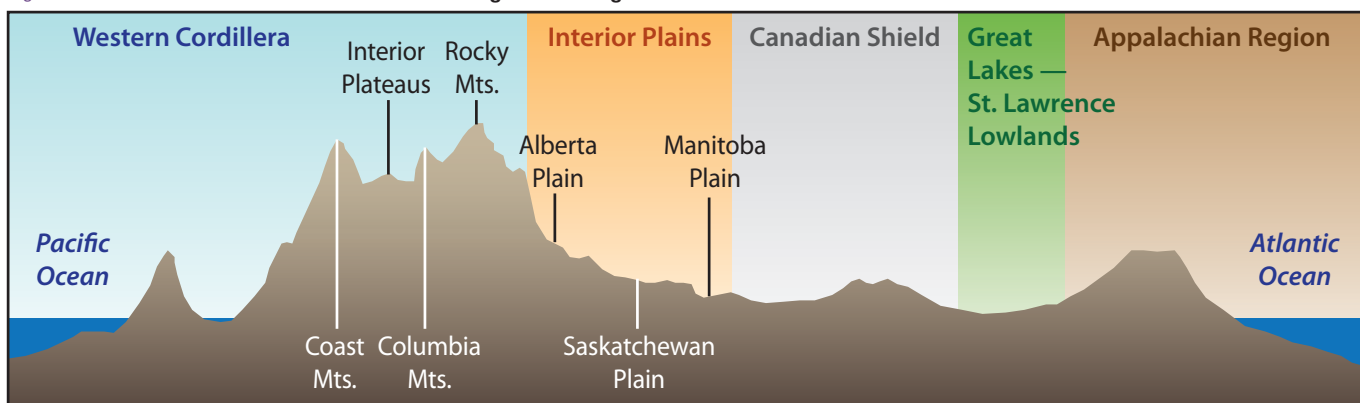
Figure 15-5 Cross-Section of Landform Regions along Canada–U.S. Border
